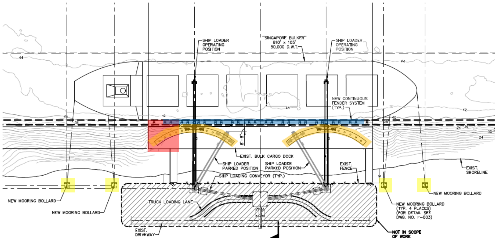
BULK CARGO DOCK AND NO. 5 DOCK SITE PLAN SCALE: 1"=50'-0"
